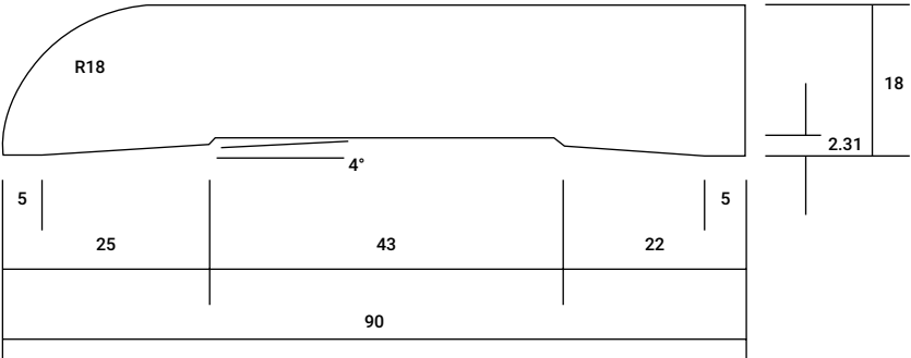
BULLNOSE AS1 90mm x 18mm
