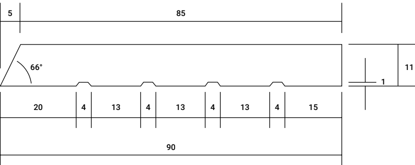
SPLAYED AS8 90mm x 11mm
