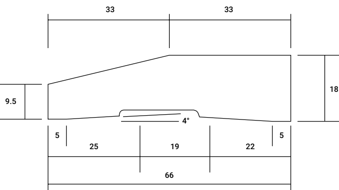
HALF SPLAYED AS5 66mm x 18mm
