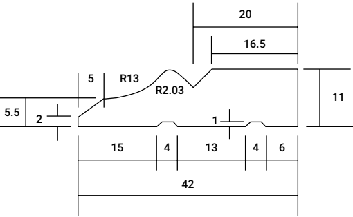
COLONIAL NSW 42mm x 11mm
