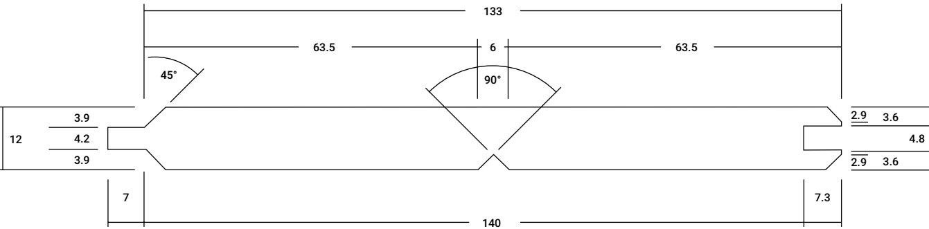
LINING 302 140mm x 12mm
