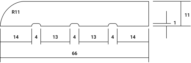
BULLNOSE AS9 66mm x 11mm
