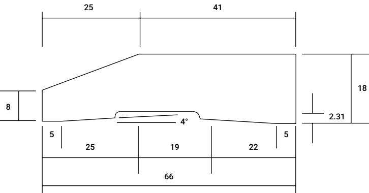
HALF SPLAYED AS4 66mm x 18mm
