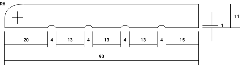
PENCIL ROUND AS15 90mm x 11mm
