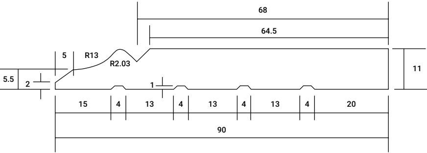
COLONIAL NSW 90mm x 11mm
