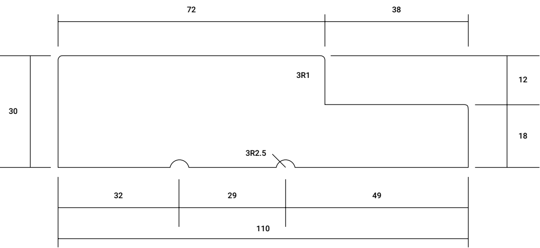
DOOR JAMB 110mm x 30mm
