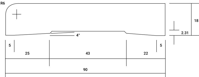
PENCIL ROUND AS7 90mm x 18mm
