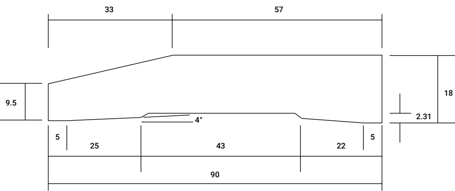
HALF SPLAYED AS5 90mm x 18mm
