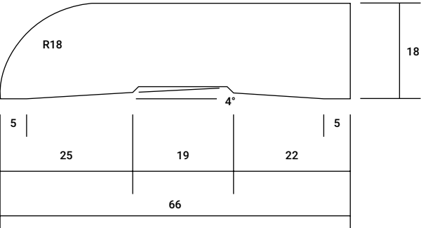
BULLNOSE AS1 66mm x 18mm
