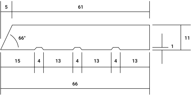
SPLAYED AS8 66mm x 11mm
