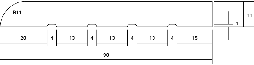
BULLNOSE AS9 90mm x 11mm
