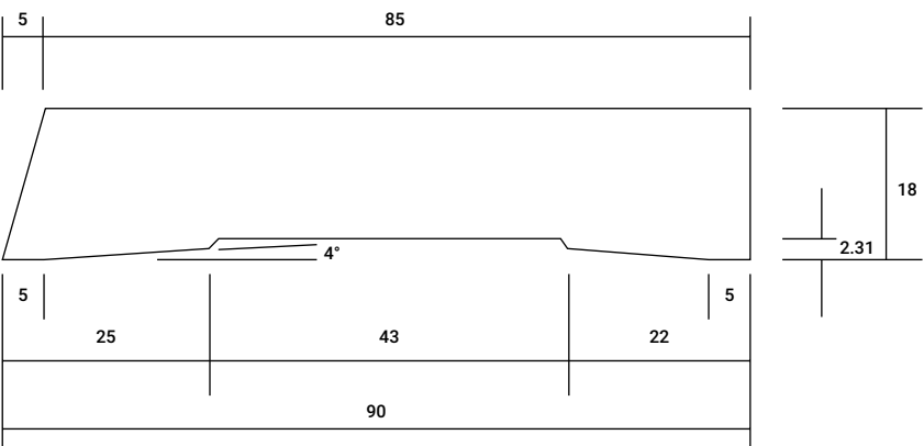
BEVEL AS3 90mm x 18mm
