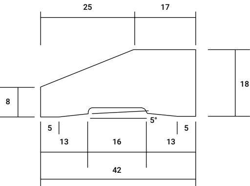
HALF SPLAYED AS4 42mm x 18mm
