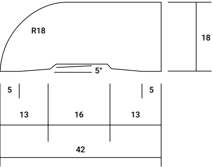
BULLNOSE AS1 42mm x 18mm
