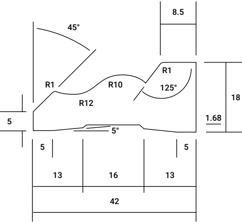
COLONIAL AS2 42mm x 18mm
