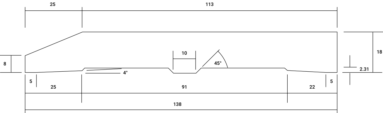
HALF SPLAYED AS4 138mm x 18mm
