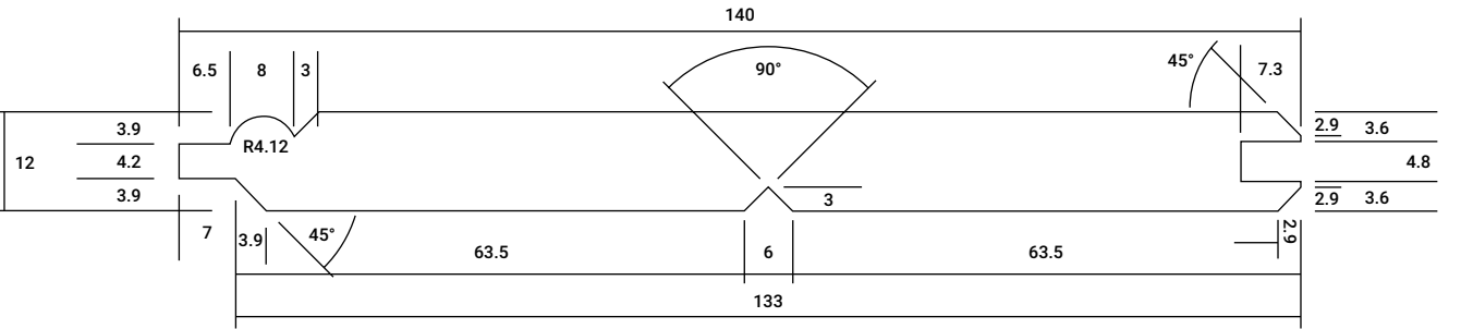
LINING 321 140mm x 12mm
