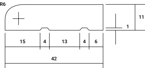
PENCIL ROUND AS15 42mm x 11mm
