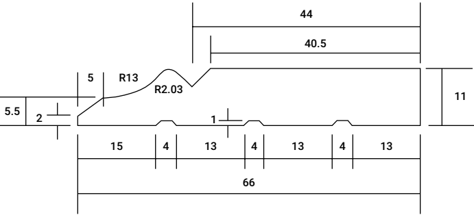
COLONIAL NSW 66mm x 11mm
