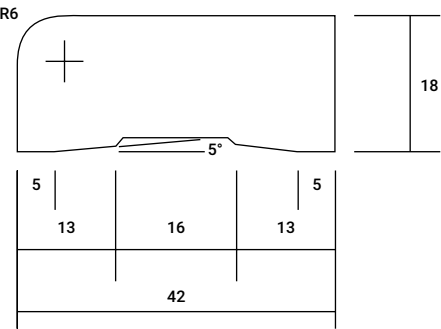
PENCIL ROUND AS7 42mm x 18mm
