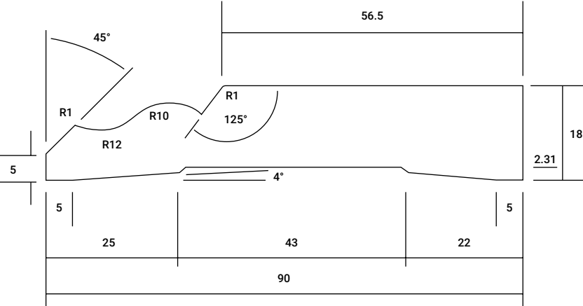
COLONIAL AS2 90mm x 18mm
