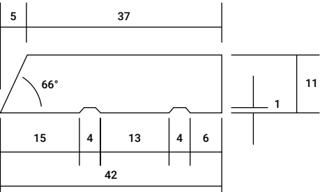
SPLAYED AS8 42mm x 11mm
