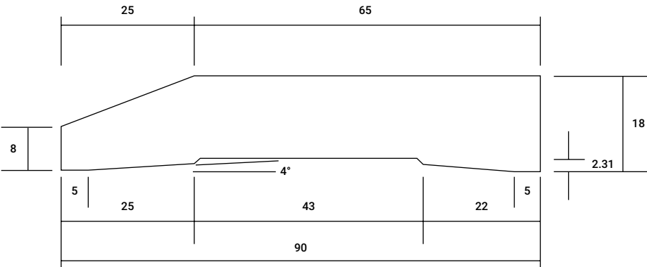
HALF SPLAYED AS4 90mm x 18mm
