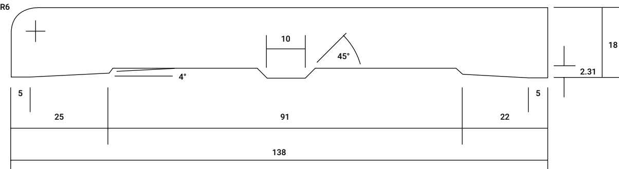
PENCIL ROUND AS7 138mm x 18mm
