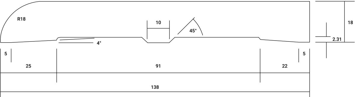
BULLNOSE AS1 138mm x 18mm
