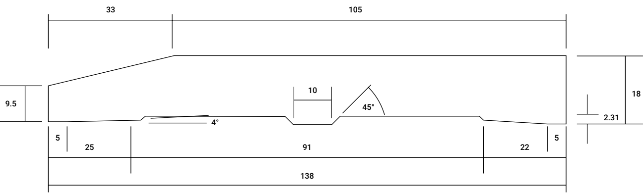
HALF SPLAYED AS5 138mm x 18mm
