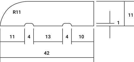
BULLNOSE AS9 42mm x 11mm
