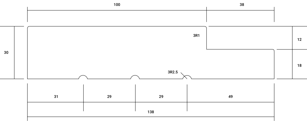
DOOR JAMB 138mm x 30mm
